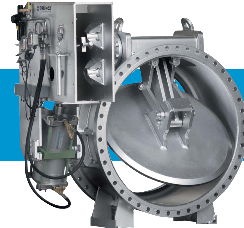
MP Three-lever valve
